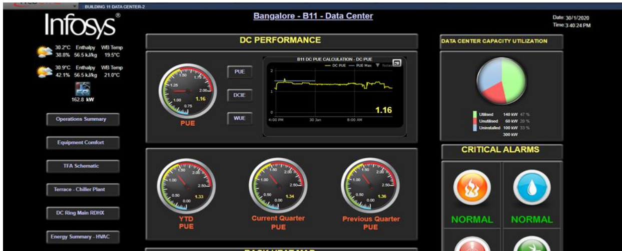
Figure 5. A main console for the building management system in the Infosis-Bangalore data center
