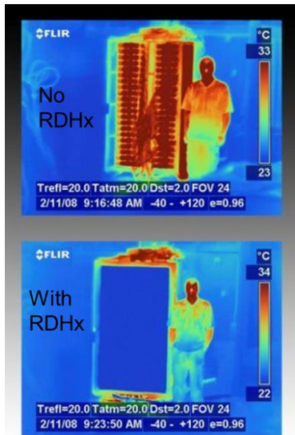
Figure 4. Infrared imagery of a RDHx system
