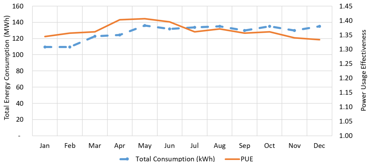
Figure 6. Monthly total energy consumption and PUE in 2019 for the Infosis-Bangalore data center
